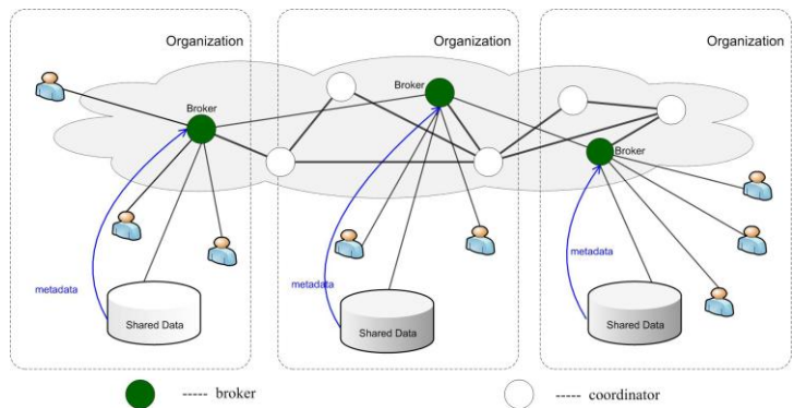
Fig.2. Architecture of PPIB
