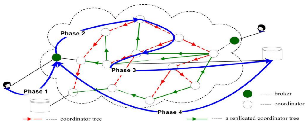
Fig. 3. Query brokering process in 4 phases.
