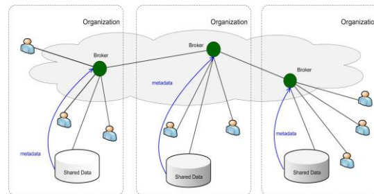
Fig.1. Overview of the IBS infrastructure.
