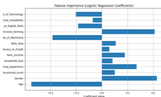
Figure no 2: Shows the feature importance (logistic regression coefficients)
