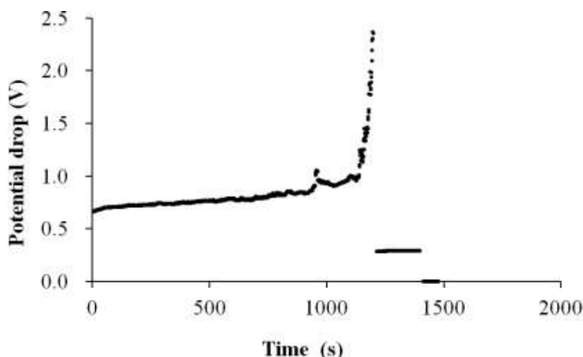
Figure 5: Voltage (V) vs. time (s) of application of current density ( 9 \text{ MA/cm}^2 ) and temperature (613 K) utilization of EM and grown as thin wire.
