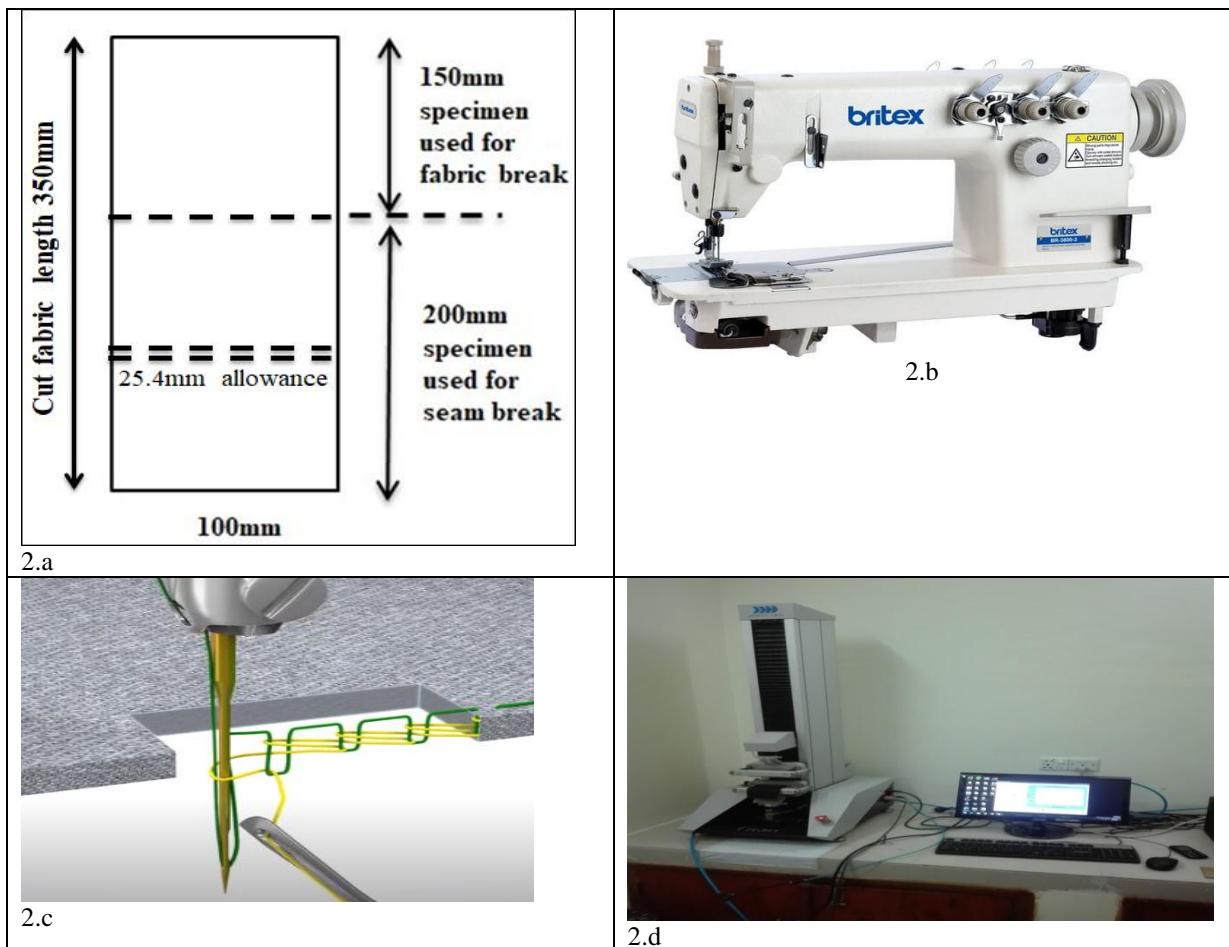
Figure 2: a. Cut fabric and seamed fabric dimension, b. Chain stitch sewing machine, c. 401 chain stitch diagram, d. Titan Universal Strength Tester
