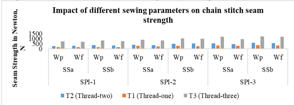
Figure 3: Impact of different sewing parameters on chain stitch seam strength
