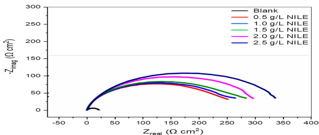
Figure 2. Effect of Napoleoniae imperialis leaves extract on mild steel coupons in 0.5M HCl
