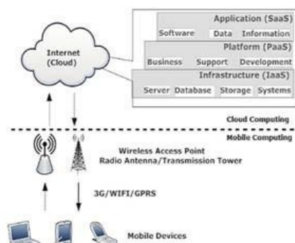
Fig 3. Mobile Cloud Computing (MCC) Architecture.
