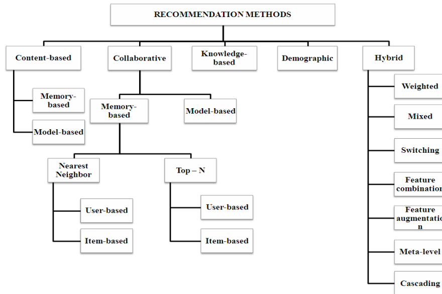
Fig. 2. Classification of recommendation methods
