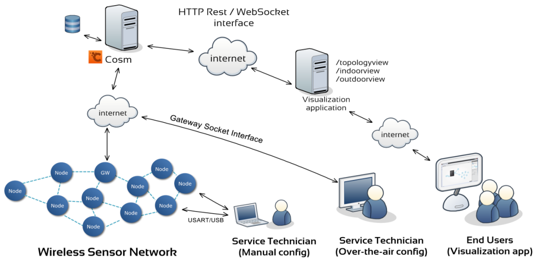
Figure 1. The general block diagram of a web enabled WSN.
