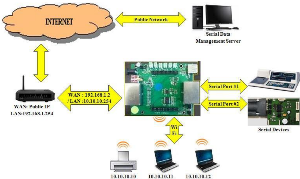
Figure 6. The EWS working in an Ad-Hoc wireless mode
