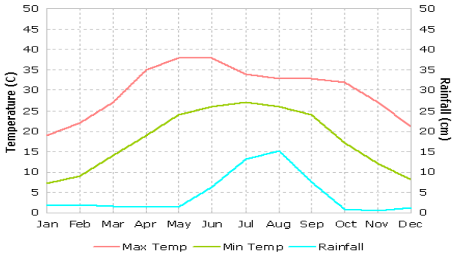
Fig 14: Average temperature rainfall analysis of Pauri
