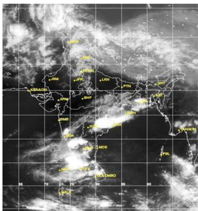
Fig 4: Satellite images before cloudburst at Leh
