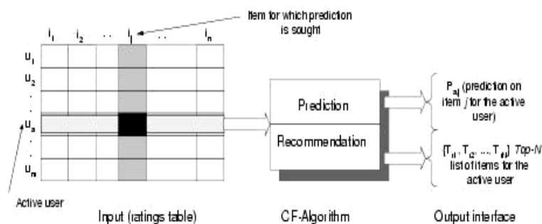
Fig.2 the Collaborative Filtering Process
