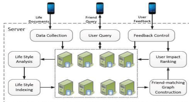
Fig1: Architecture
