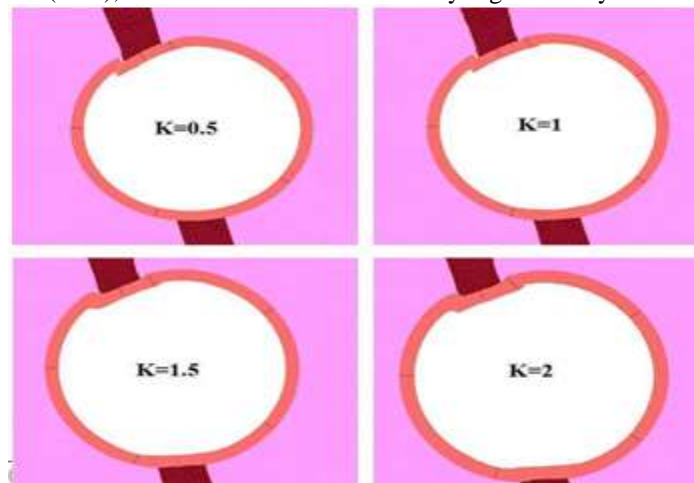
Figure 8. Deformation of the segmental lining at different stress fields
