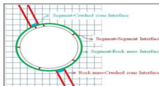
Figure 6. Different interfaces in numerical modeling
