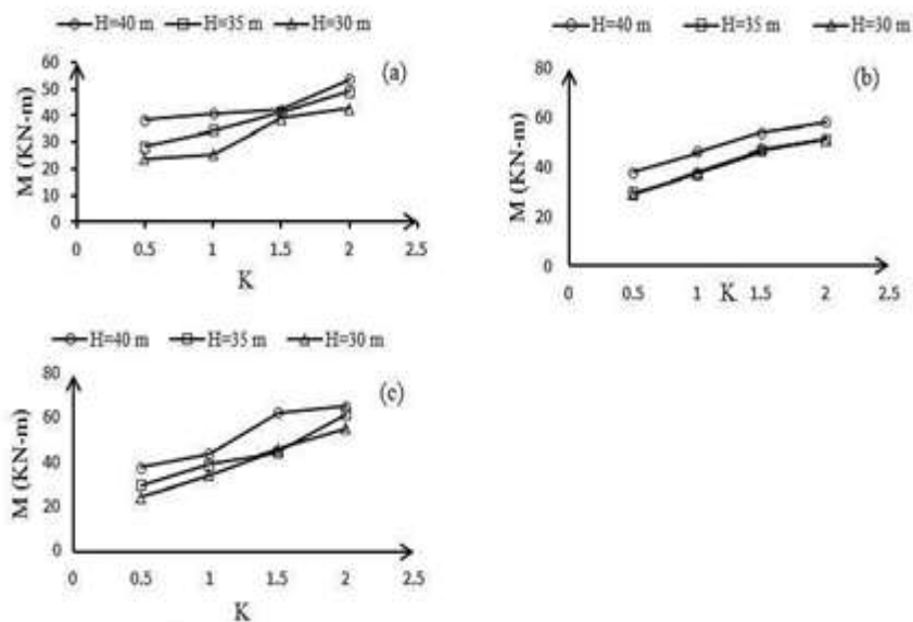
Figure 10. Induced bending moment in longitudinal joint at the location of the key segment and the crushed zone interface a) Marl b) Shale c) Sandstone
