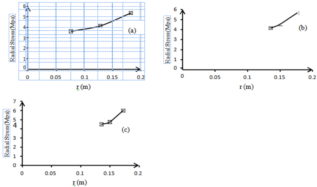
Figure 13. Induced radial stress vs. joint opening length for different material properties a) Marl b) Shale c) Sandstone
