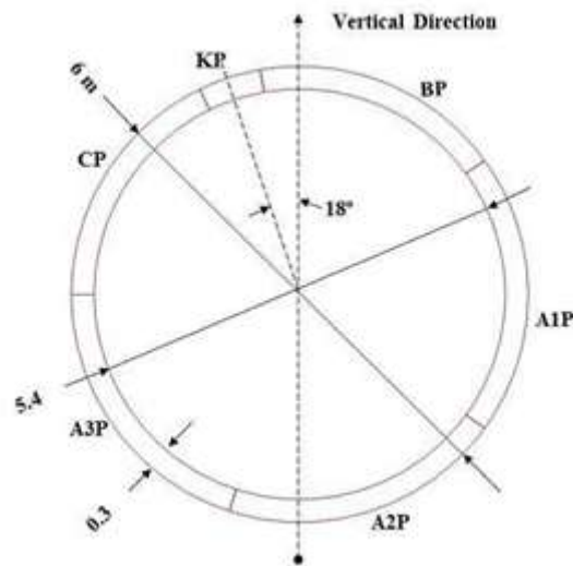
Figure 2. Segment arrangement and numbering
