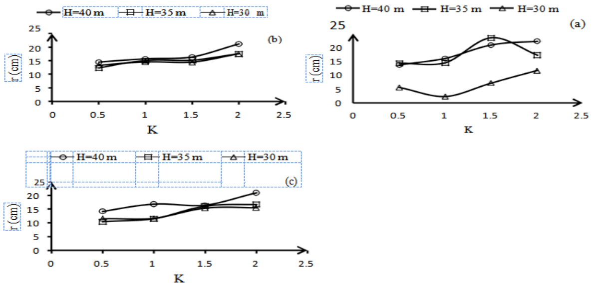
Figure 12. Relationship between the coefficient of stress concentration and opening length at the location of the key segment and the crushed zone interface a) Marl b) shale c) sandstone
