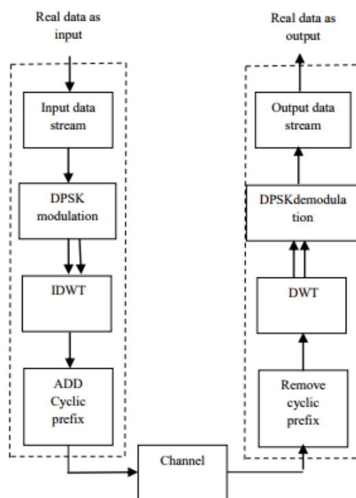
Figure 2: Extension method block diagram for data transfer using DWT
