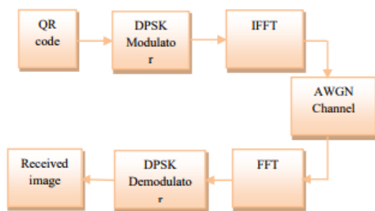
Figure 1: Transmission of information using DPSK Algorithm
