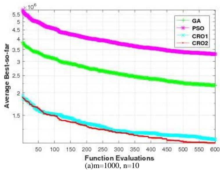
Figure 1.2: Comparison of GA, PSO, CRO1, and CRO2 on the MCKP. The objective function value ere averaged over 25 runs
