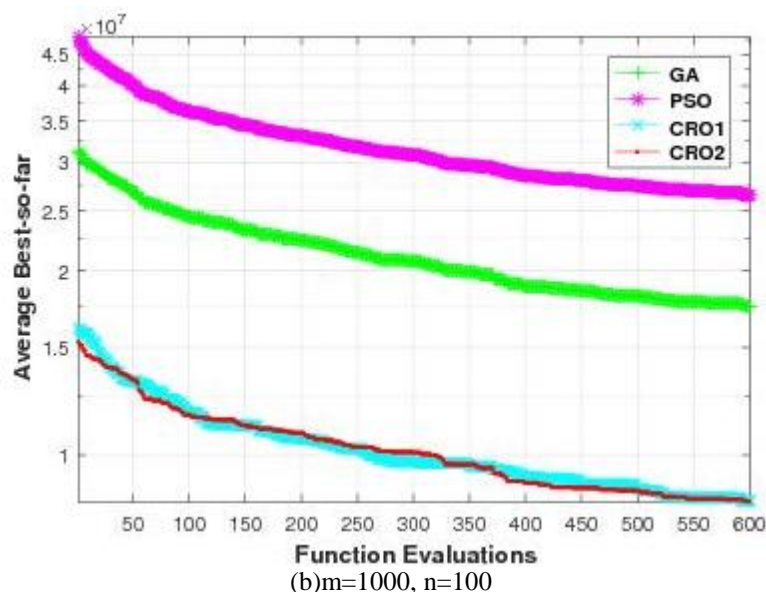
Figure 1.3: Comparison of GA, PSO, CRO1, and CRO2 on the MCKP. The objective function value was averaged over 30 runs
