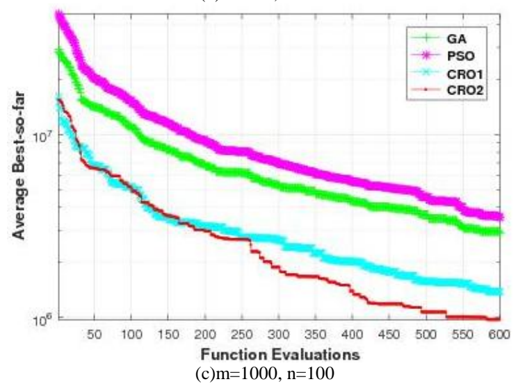
Figure 1.2: Comparison of GA, PSO, CRO1, and CRO2 on the MCKP. The objective function value ere averaged over 25 runs
