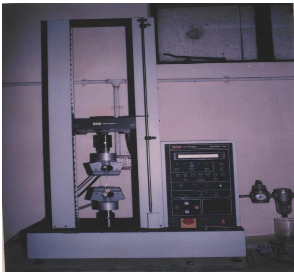
Fig-5 :Universal testing machine (Model 1104 Instron Co) Fig-6 :Specimen in universal testing machine
