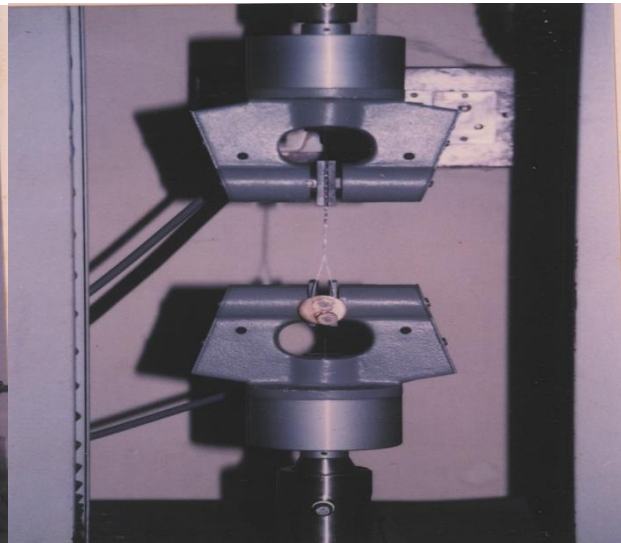
Fig-5 :Universal testing machine (Model 1104 Instron Co) Fig-6 :Specimen in universal testing machine
