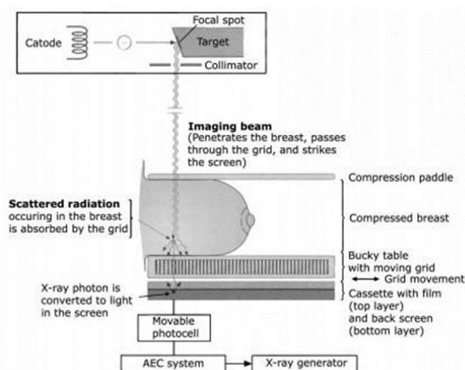
Fig. 2.5: Schematic Diagram of Mammographic System [73].
