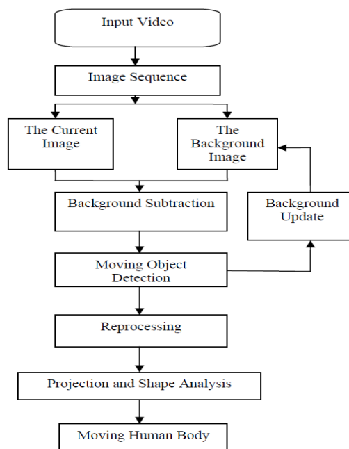
Figure 1: The Flowchart of Moving human Body Extraction
