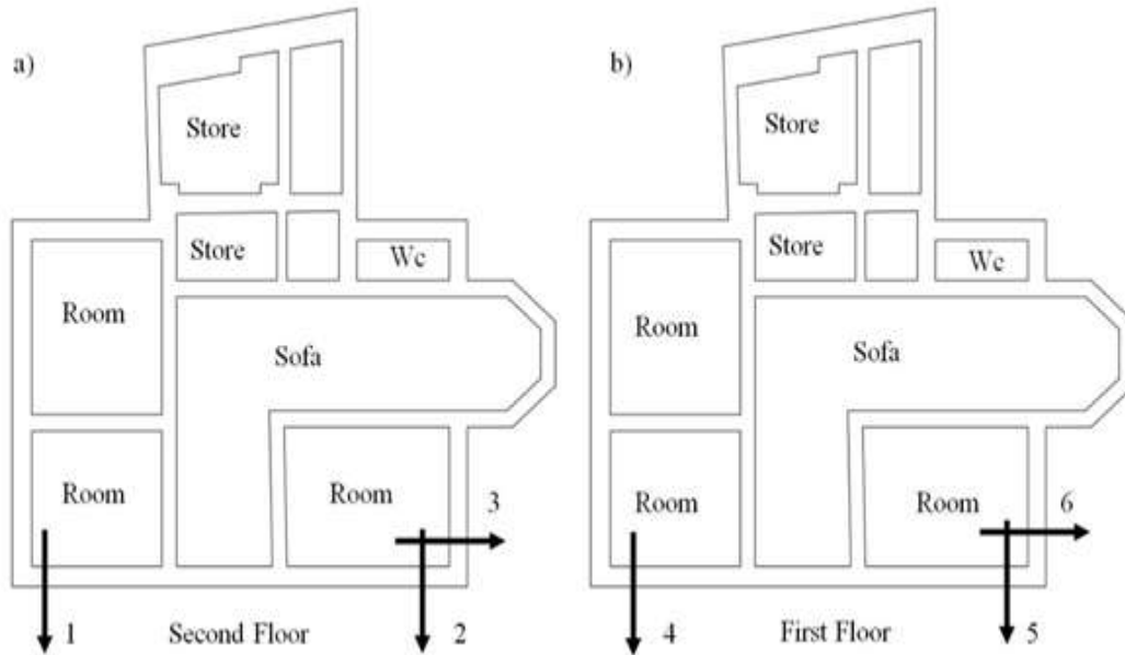
Figure 9. The sensor orientations on plan views a) Second floor b) First floor
