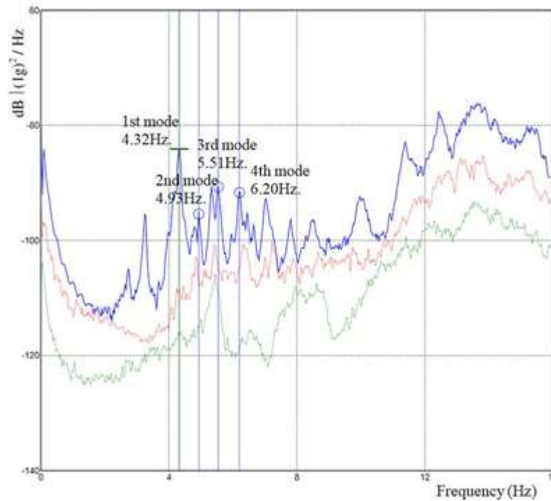
Figure 11. The singular values of the spectral densities
