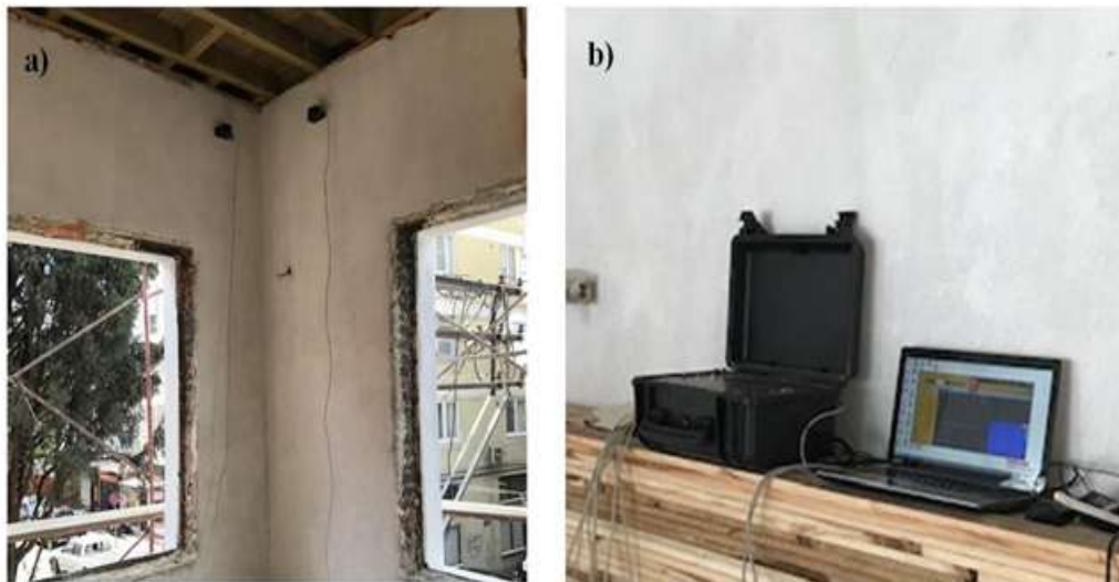
Figure 10. The sensor placements and the test equipment
