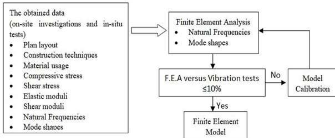
Figure 1. The flowchart of the study
