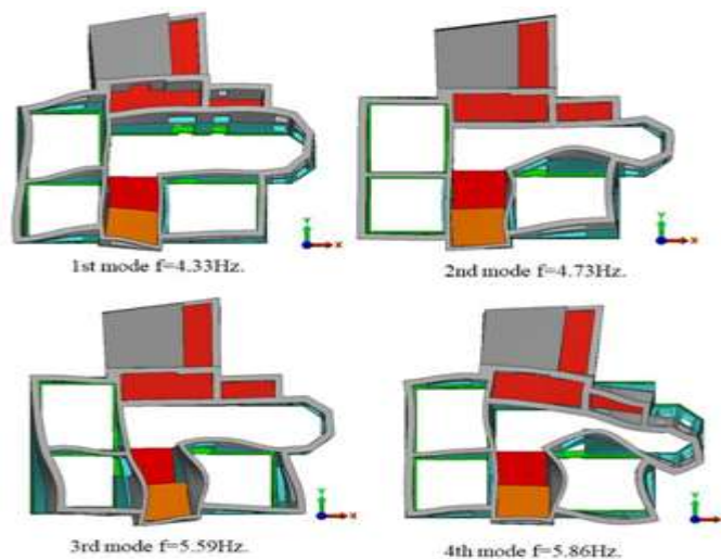
Figure 12. The first four mode shapes and frequencies
