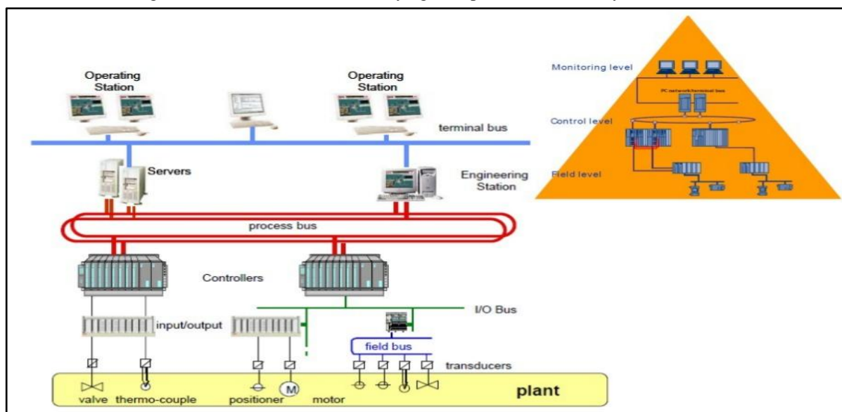
Fig. 1 DCS Structure
