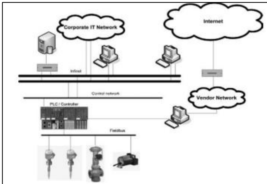
Fig. 8 Network Bridge
