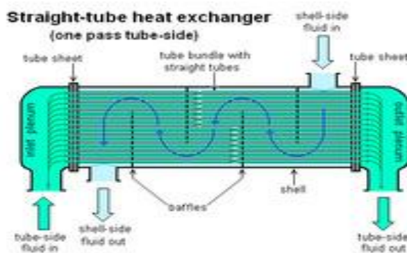
Fig.1.2: Shell and tube heat exchanger
