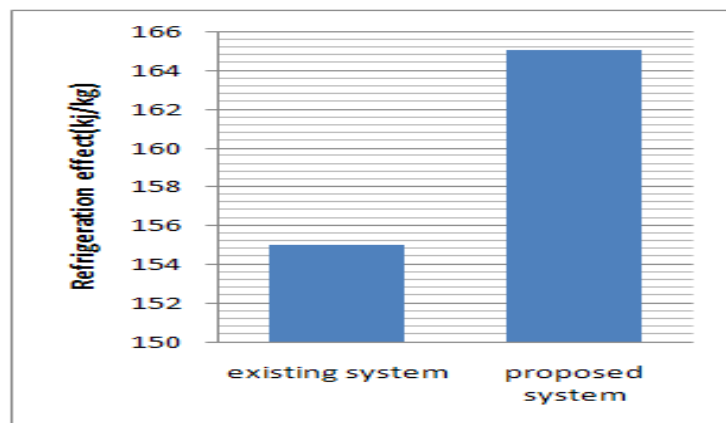
Graph 2 Comparison of net refrigeration effect for existing system and proposed system
