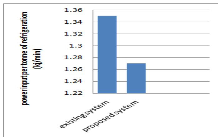
Graph 3 Comparison of power input per tonne of refrigeration for existing system and proposed system
