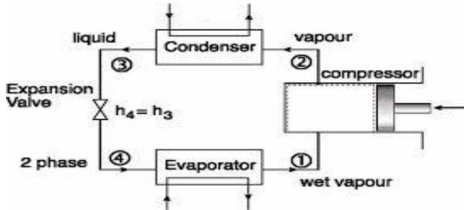
Fig. 1.1 vapor compression refrigeration system
