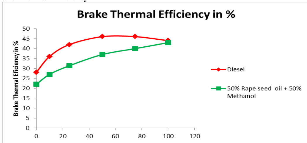
Fig-3 shows the variations of Brake Thermal Efficiency for Diesel and Rape seed oil blended with Methanol at different Loads
