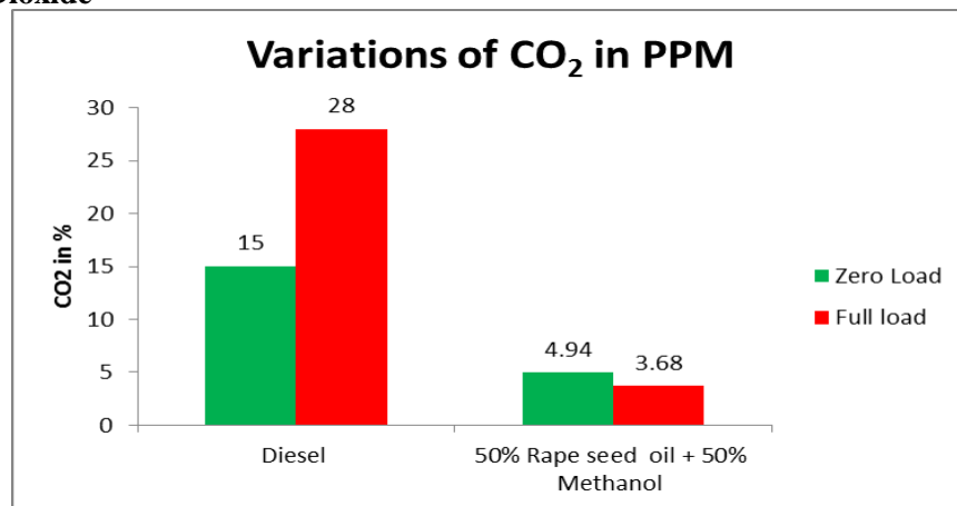
Fig-5 shows the variations of Carbon dioxide for Diesel and Rape seed oil blended with Methanol at Zero Load and Full Load
