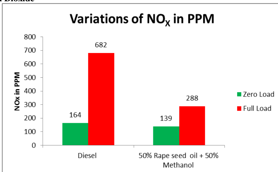
Fig-6 shows the variations of Nitrogen dioxide for Diesel and Rape seed oil blended with Methanol at Zero Load and Full Load
