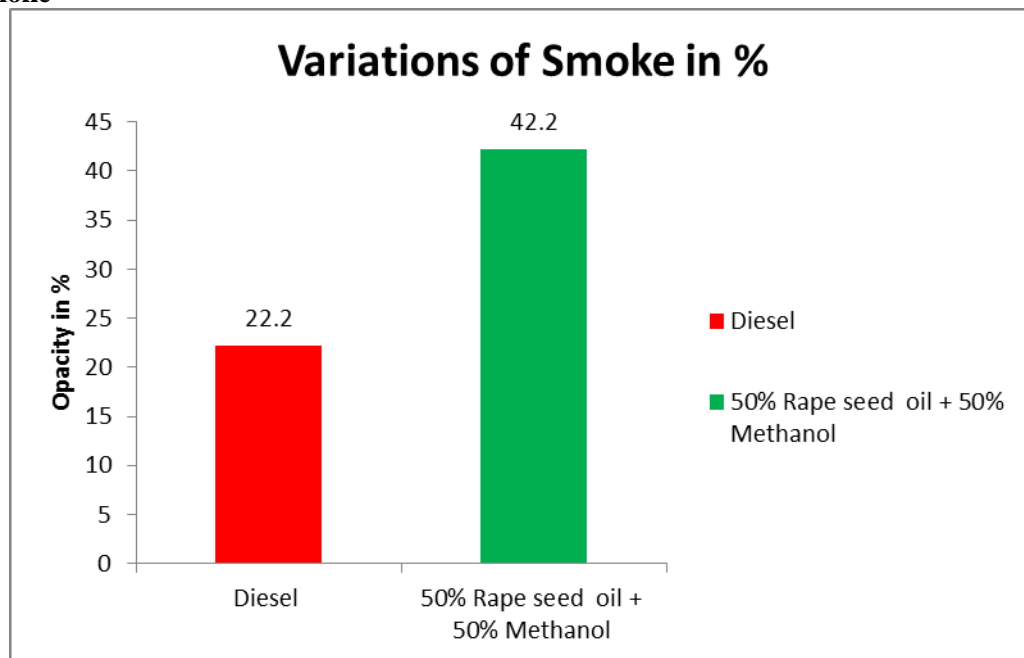
Fig-7 shows the variations of Smoke for Diesel and Rape seed oil blended with Methanol at Zero Load and Full Load
