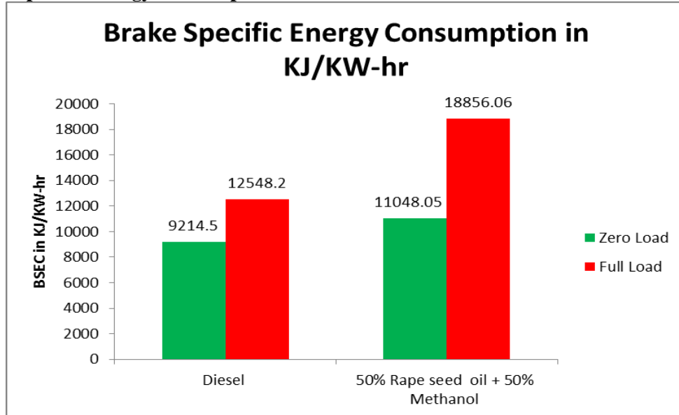
Fig-2 shows the variations of Brake Specific Energy Consumption for Diesel and Rape seed oil blended with Methanol at Zero Load and Full Load
