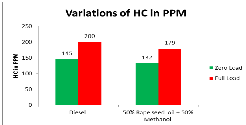
Fig-4 shows the variations of Unburnt Hydro Carbon for Diesel and Rape seed oil blended with Methanol at Zero Load and Full Load
