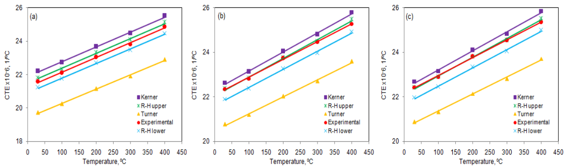
Figure 4: Coefficient of thermal expansion as a function of temperature for AA1100/5% vf: (a) 100% ZrO 2 , (b) 85% ZrO 2 doped with 8% Y 2 O 3 and (c) 85% ZrO 2 doped with 15% Y 2 O 3 .
