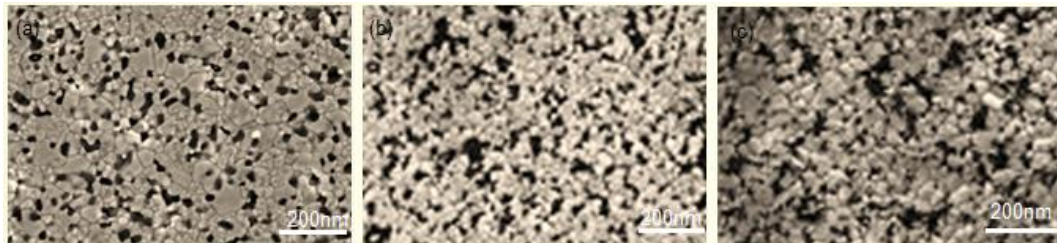
Figure 4: Microstructures of Al/ZrO 2 composites: (a) 30 vol.% pure ZrO 2 (b) 30 vol.% ZrO 2 doped with 8% Y 2 O 3 and (c) 30 vol.% ZrO 2 doped with 15% Y 2 O 3 .
