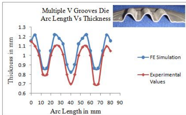
Fig. 7 Multiple V Groove Die: Arc Length Vs Thickness
