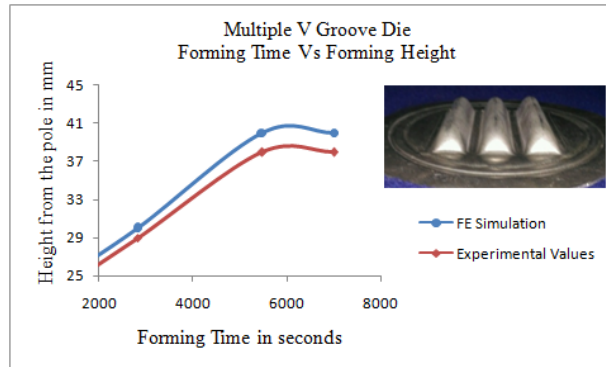
Fig. 6 Multiple V Groove Die: Forming Time Vs Forming Height
