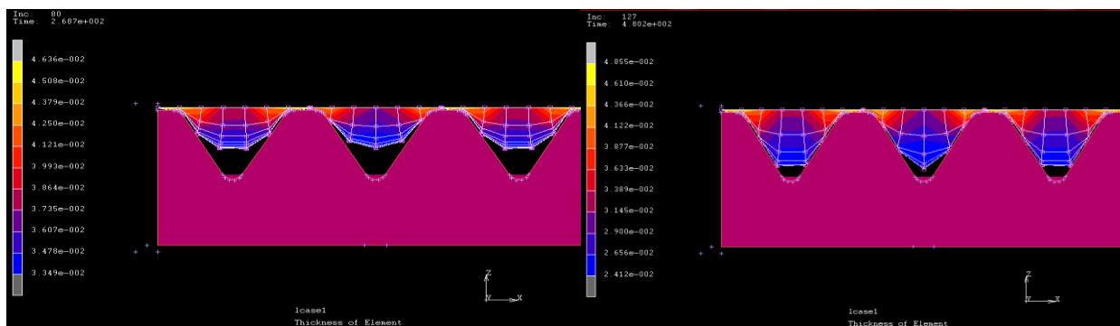
Fig (c): Deformation distribution of sheet at stage 3
