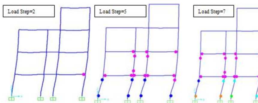
Figure 9: Plastic hinge patterns at different load steps on Building before dismantling (Building 1).
