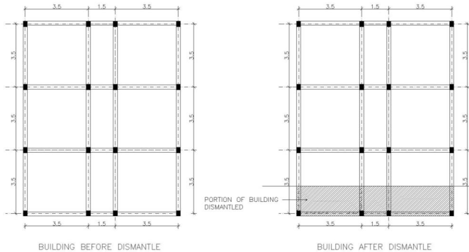
Figure 2: Building type 1 before and after dismantling.
