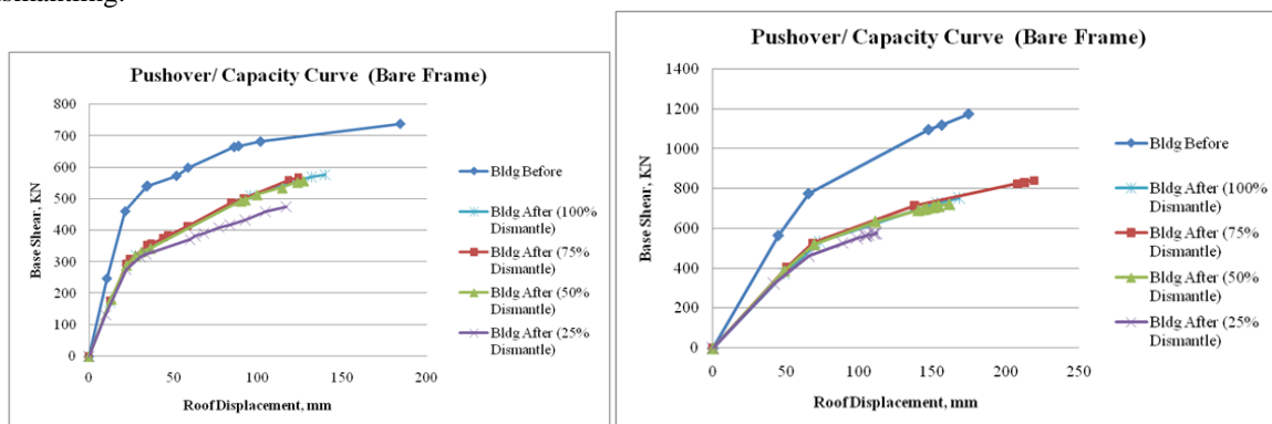
Figure 5: Pushover/Capacity curve (Building 1 and Building 2).
