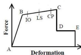
Figure 4: Typical Capacity Curve.
