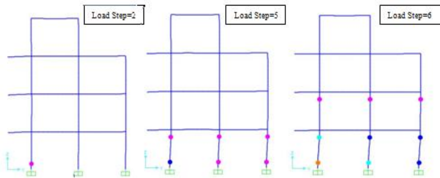
Figure 10: Plastic hinge patterns at different load steps on 50% dismantling (Building 1).
