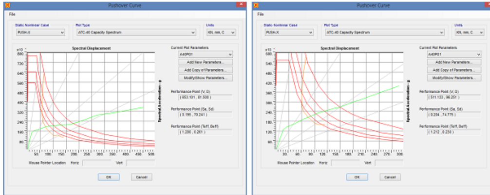
Figure 6: ATC-40 Capacity Curve for Building before and after 75% dismantling.
