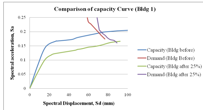
Figure 8: Comparison of ATC 40 capacity curve before and after 25% dismantle
