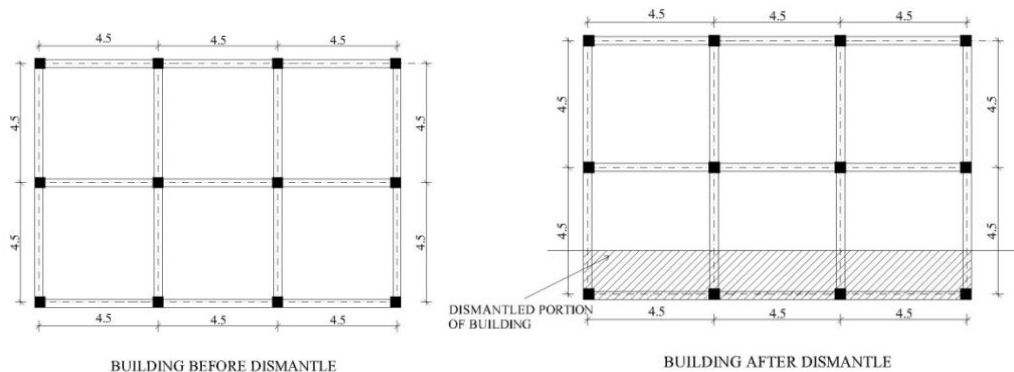
Figure 3 Building type 2 before and after dismantling.
