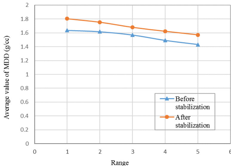
Fig.1 Effect of lime on MDD before and after stabilization.
