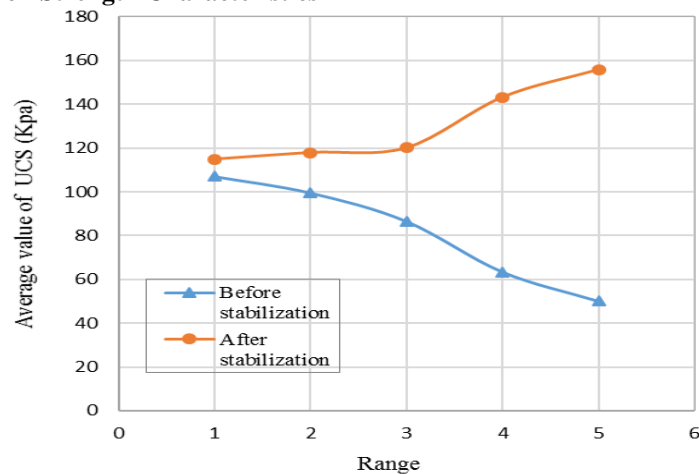
Fig. 3 Effect of lime on UCS before and after stabilization.
