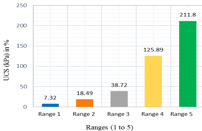
Fig. 4 Strength improvement after stabilization with lime.
