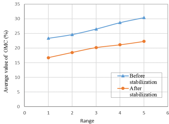
Fig.2 Effect of lime on OMC before and after stabilization.
