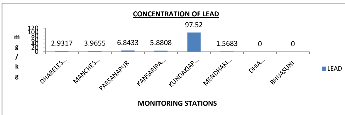
(Figure7.Comparative Graph of Lead Content in Collected Macro-algae from Different stations)
