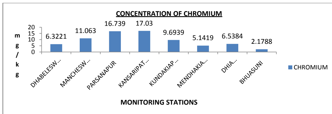
(Figure5. Comparative Graph of Chromium Content in Collected Macro-algae from Different stations)
