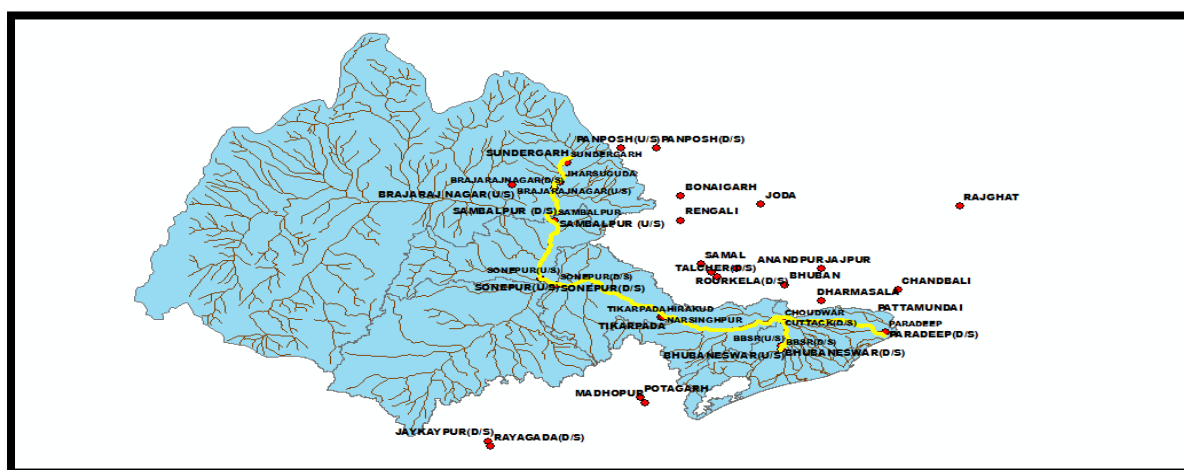
(Figure 1. Monitoring stations of River Mahanadi showing the flow path)
