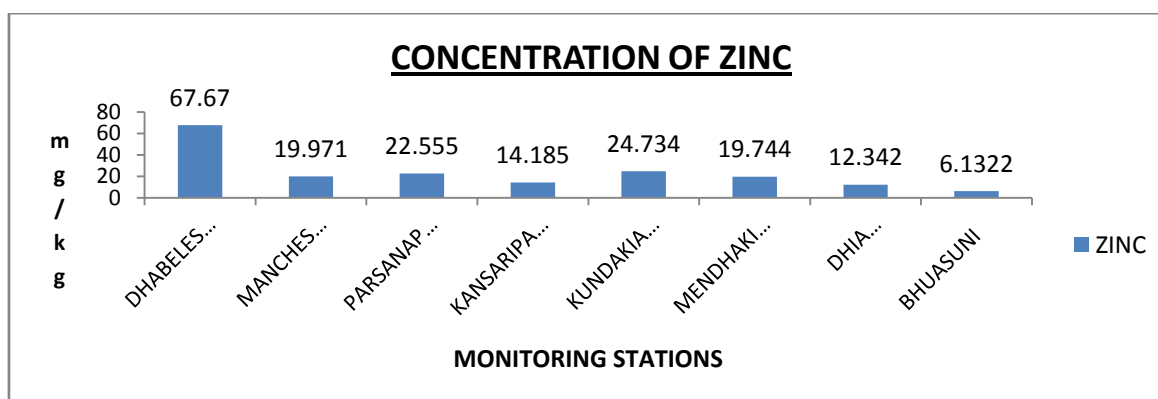
(Figure8.Comparative Graph of Zinc Content in Collected Macro-algae from Different stations)
