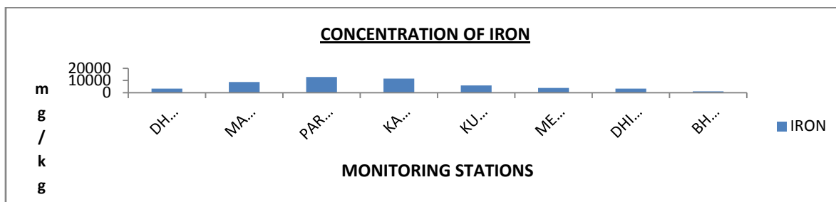
(Figure6.Comparative Graph of Iron Content in Collected Macro-algae from Different stations)
