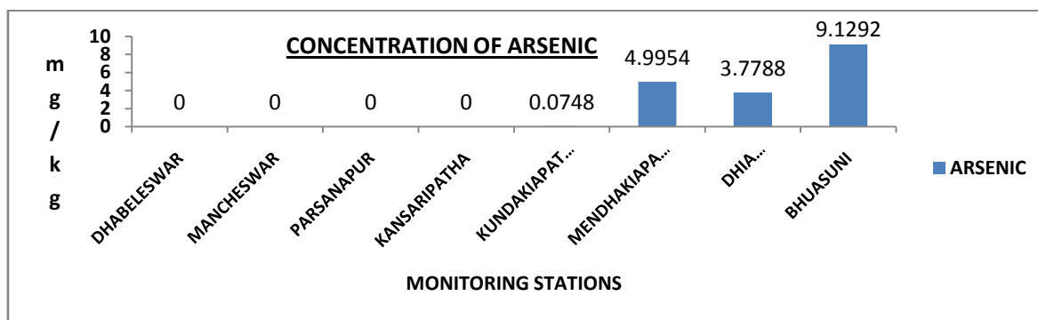
(Figure4. Comparative Graph of Arsenic Content in Collected Macro-algae from Different stations)
