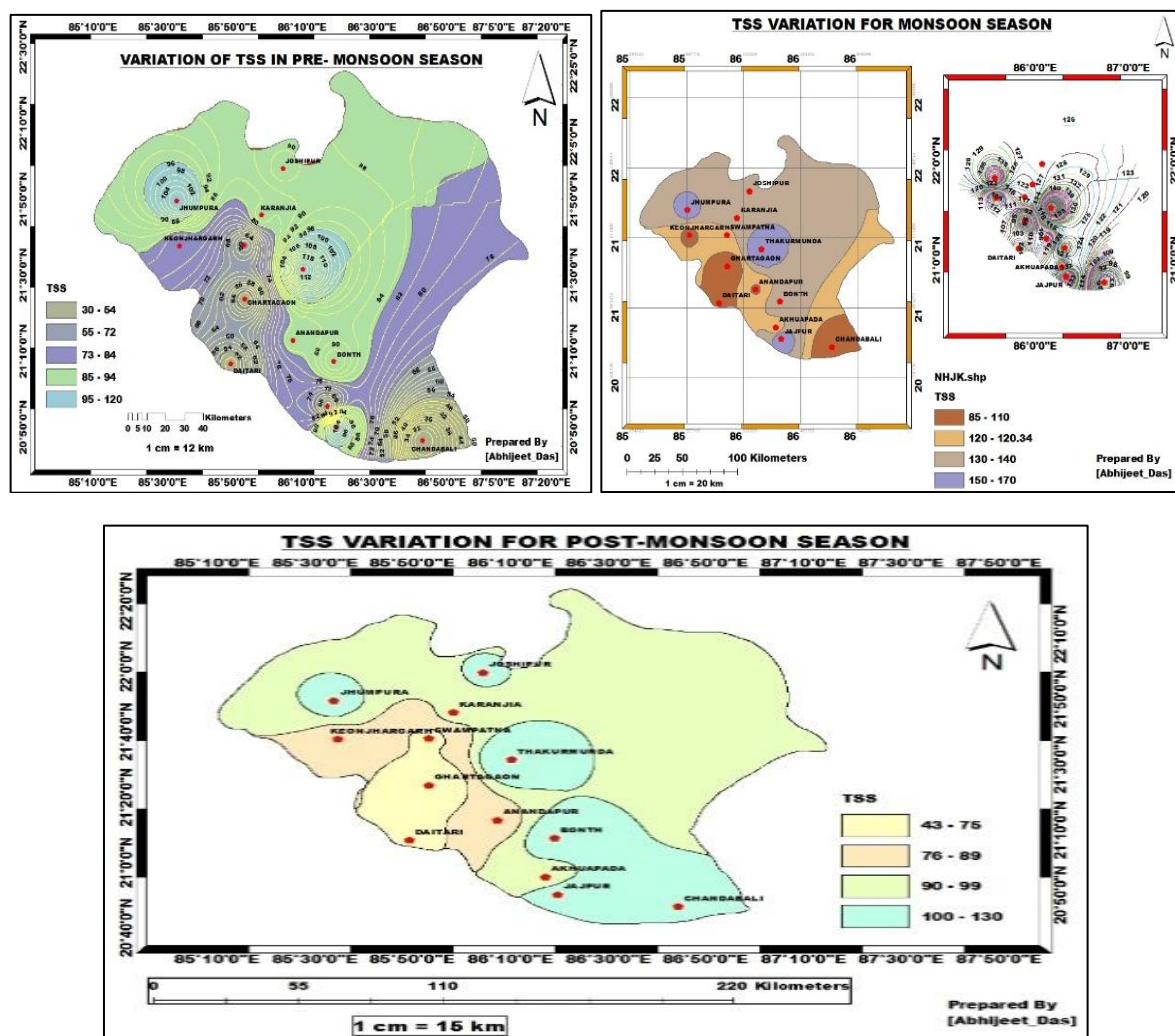
(Figure 8. Spatial variations of TSS in pre-monsoon, monsoon and post-monsoon season)
