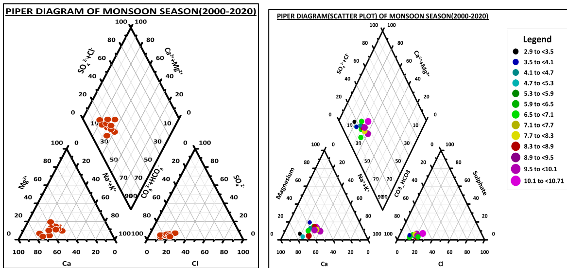
(Figure 37. Piper Diagram for monsoon season)
