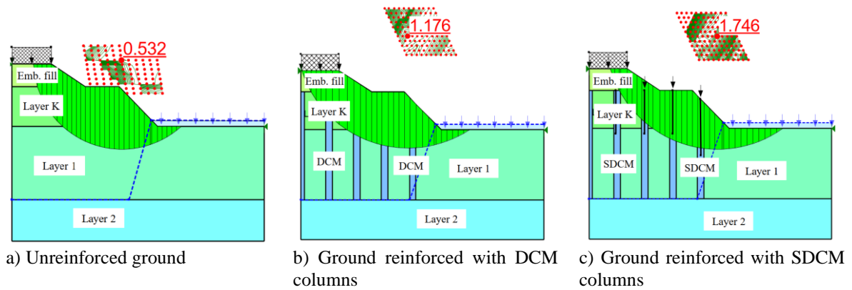
Figure 6. Factor of safety at the groundwater level of -10.0 m
