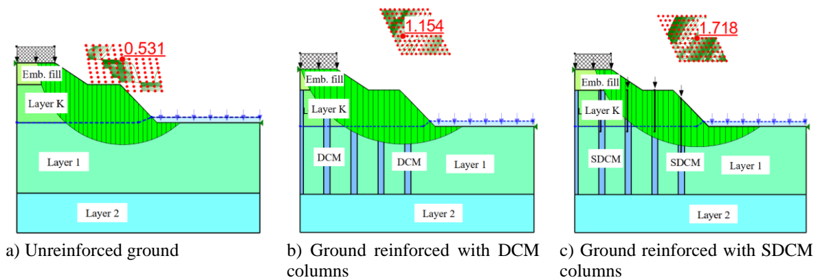
Figure 5. Factor of safety at the groundwater level of -3.5 m
