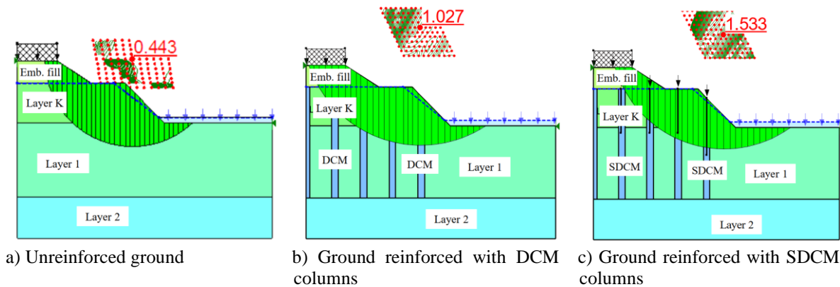
Figure 3. Factor of safety at the groundwater level of 0.0 m
