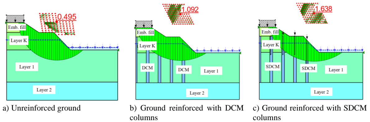
Figure 4. Factor of safety at the groundwater level of -1.5 m
