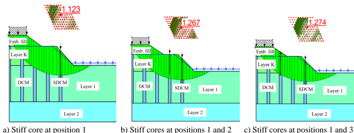
Figure 7. Factor of safety when DCM columns is reinforced with stiff core
