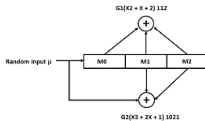
Fig. 1 Convolutional Encoder for code rate 1/2
