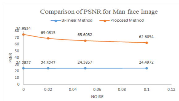
Fig. 10 Comparison of PSNR for Man's face Image
