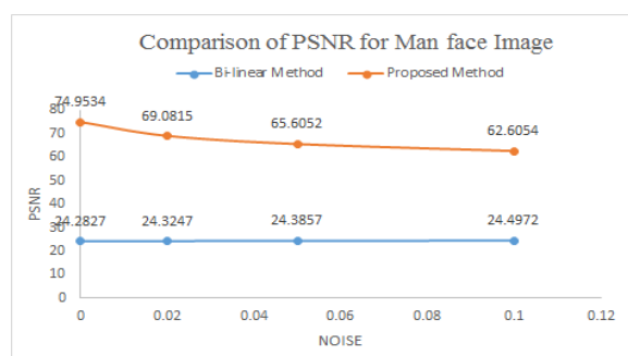
Fig. 10 Comparison of PSNR for Man's face Image
