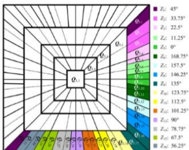
Fig. 3 Curvelet coefficient matrices at different scale and partition
