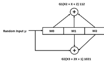
Fig. 1 Convolutional Encoder for code rate \frac{1}{2}
