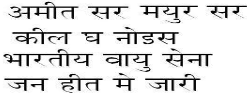
Fig.6 Line Segmentation
