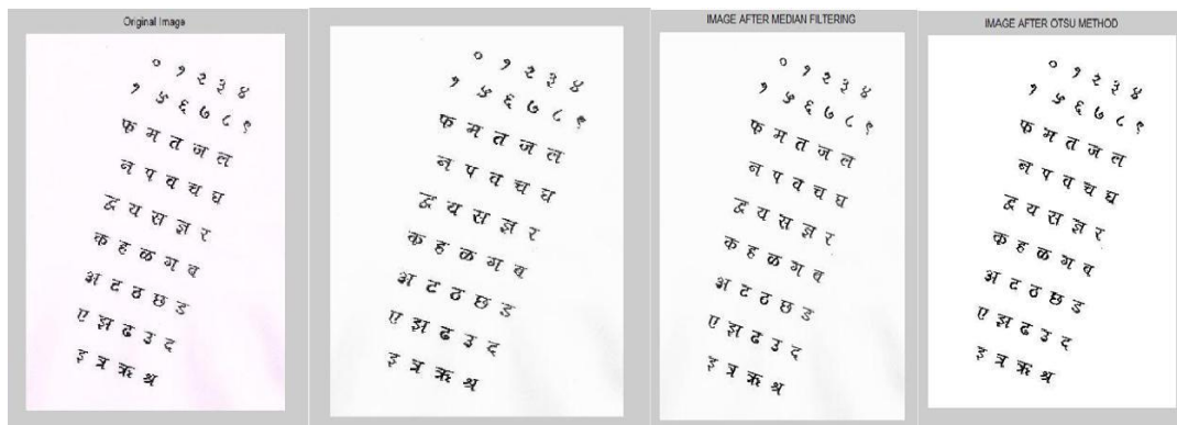
Fig.3 Pre-processing techniques
